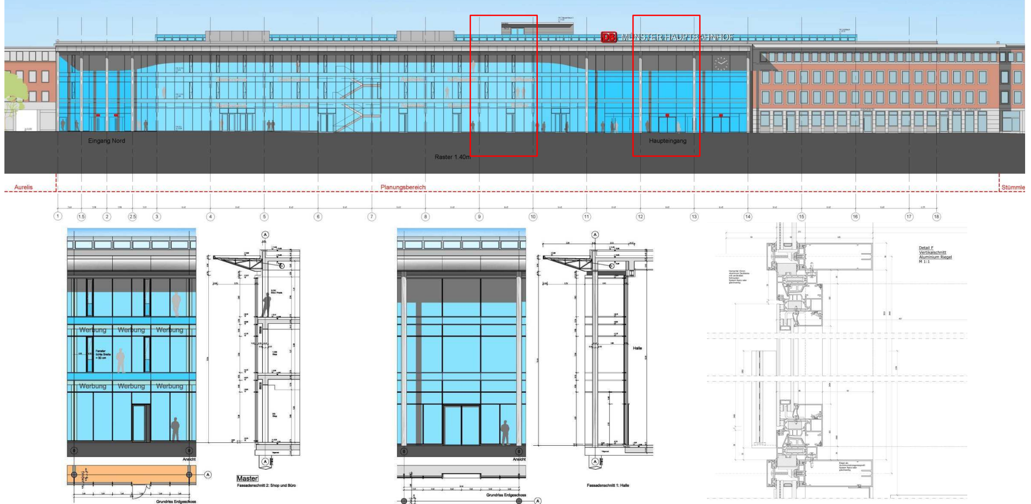
Fassade Büro/Shop
